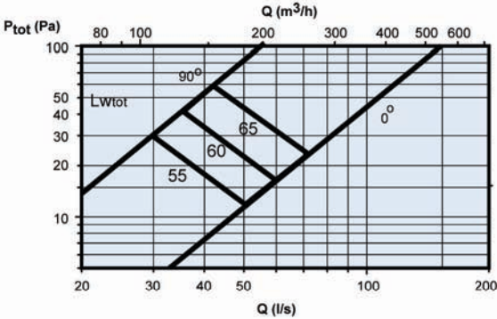
LDS.250 k=30,5 (l/s); 110 (m³/h)
