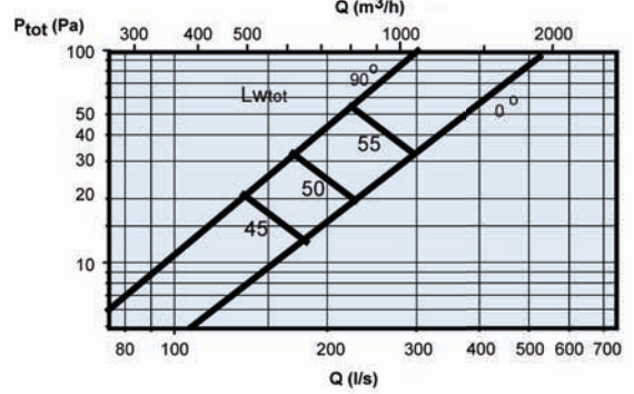
LDS.315 k=50,5 (l/s); 182 (m³/h)
